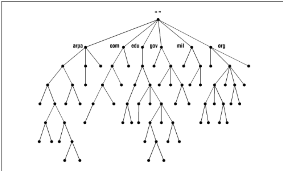
Figure 2.1: The structure of the DNS name space
