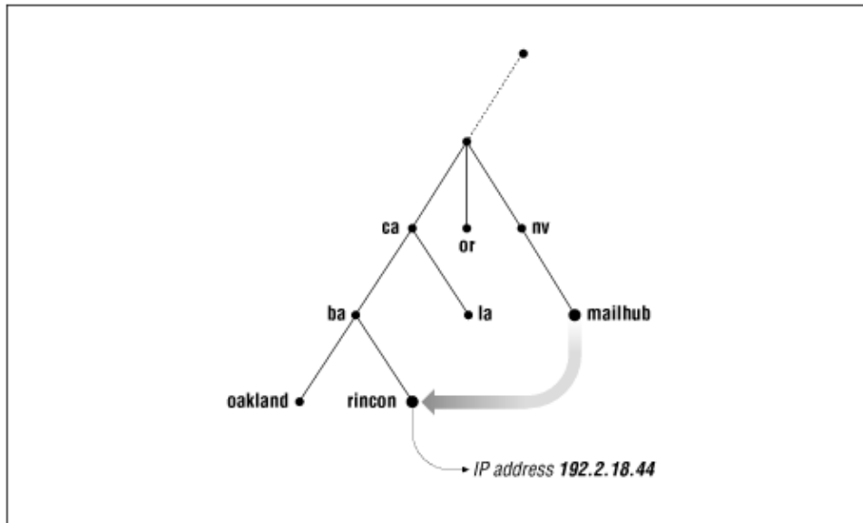
Figure 1.5: Solving the name collision problem
